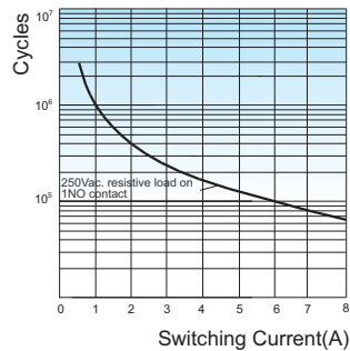
ELECTRICAL ENDURANCE
